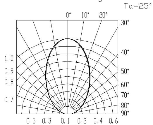
Radiation Diagram
