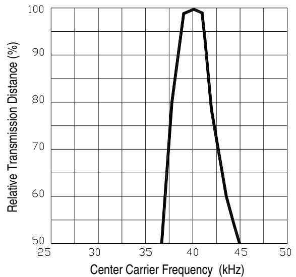
IRM-H240T/TR2
