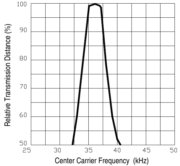
IRM-H236T/TR2
