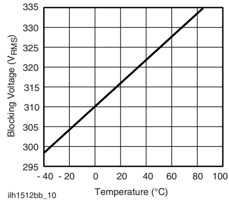
Fig. 10 - Form B Typical Blocking Voltage vs. Temperature
