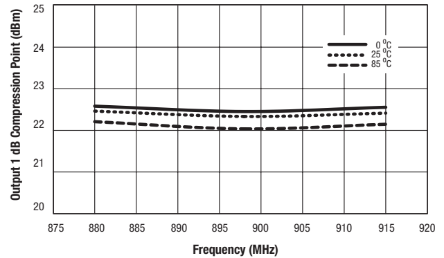
Figure 16. Mixer A OP1dB vs Frequency and Temperature
