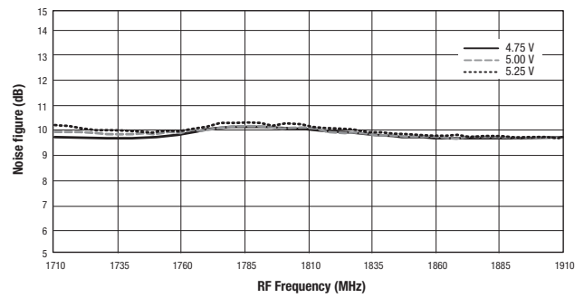
Figure 12. Mixer B Noise Figure vs Frequency and Supply Voltage
