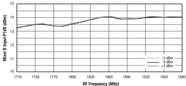
Figure 24. Mixer B Input P1dB vs Frequency and LO Power
