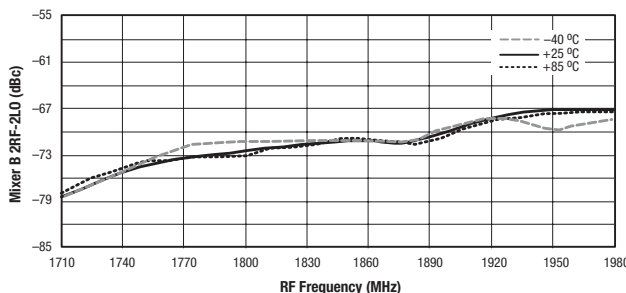
Figure 26. Mixer B 2RF-2LO vs Frequency and Temperature
