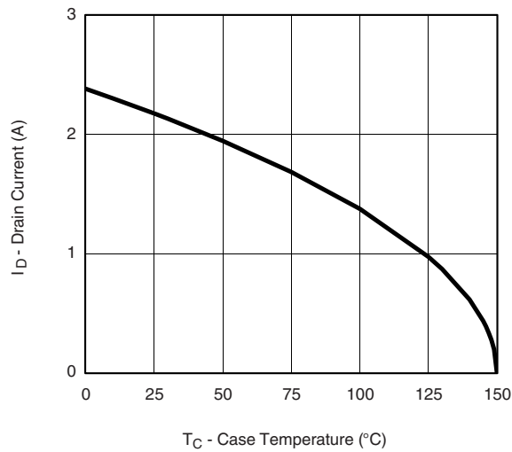
Max Current vs. Case Temperature
