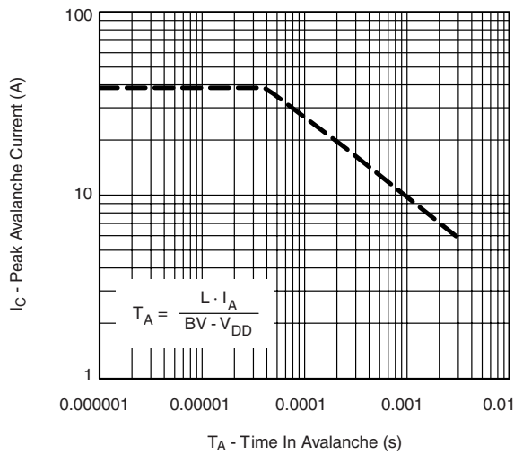
T_A - Time In Avalanche (s) Single Pulse Avalanche Capability
