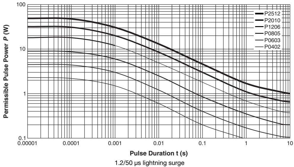
1.2/50 \mu s lightning surge
