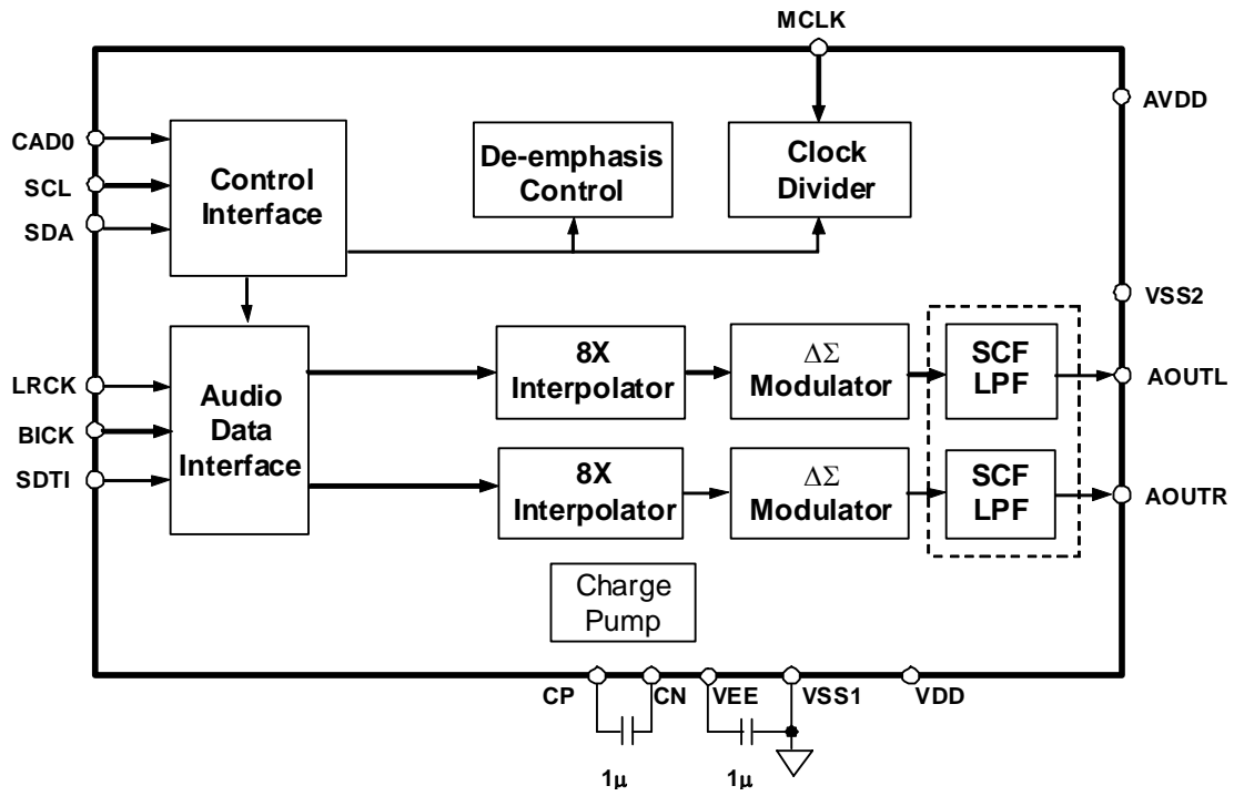
Block Diagram
