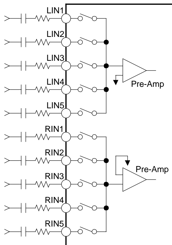
Figure 6. Input Selector
