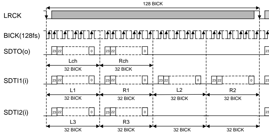
Figure 12. Mode 11 Timing
