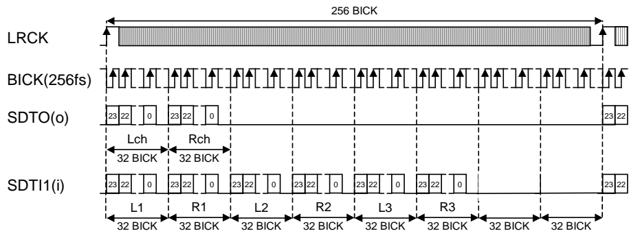
Figure 7. Mode 6 Timing
