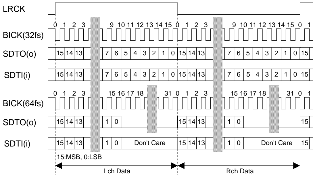
Figure 23. Mode 2 Timing
