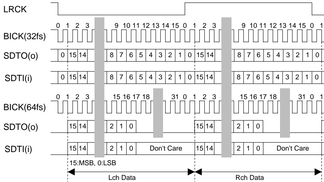
Figure 24. Mode 3 Timing
