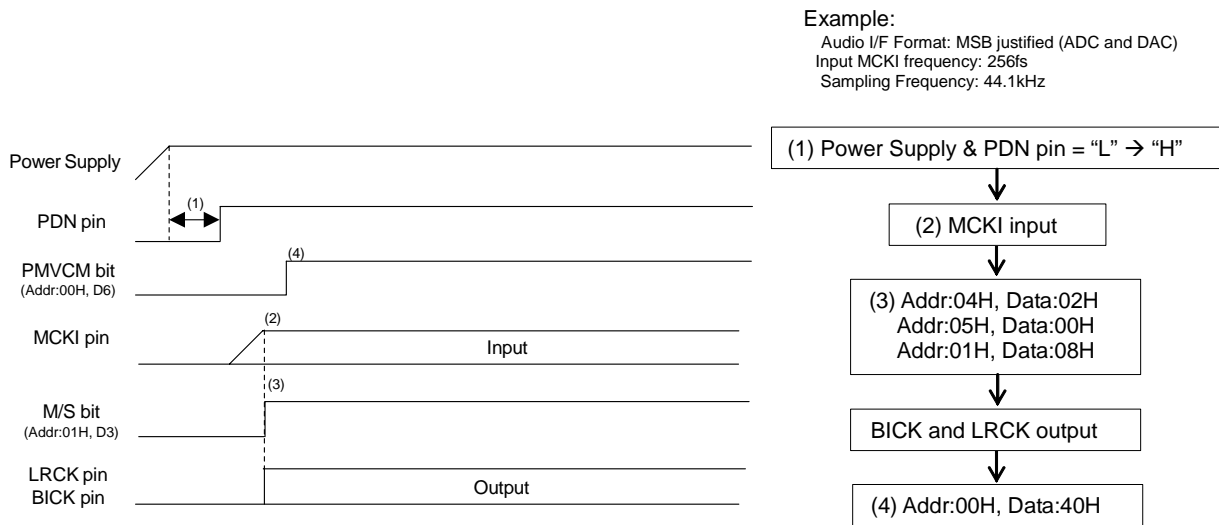
Figure 70. Clock Set Up Sequence (5)
