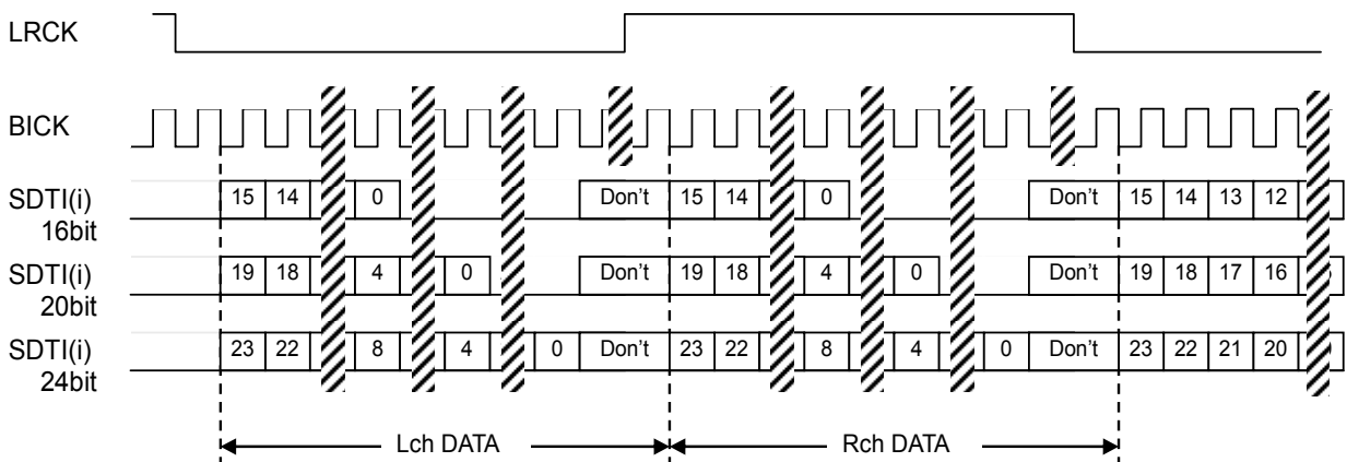
Figure 34. Mode 3 Timing
