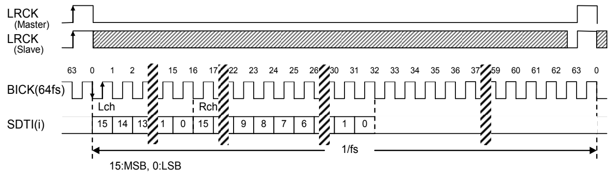
Figure 30. Mode 0 Timing (BCKP bit=“1”, MSBS bit=“1”)
