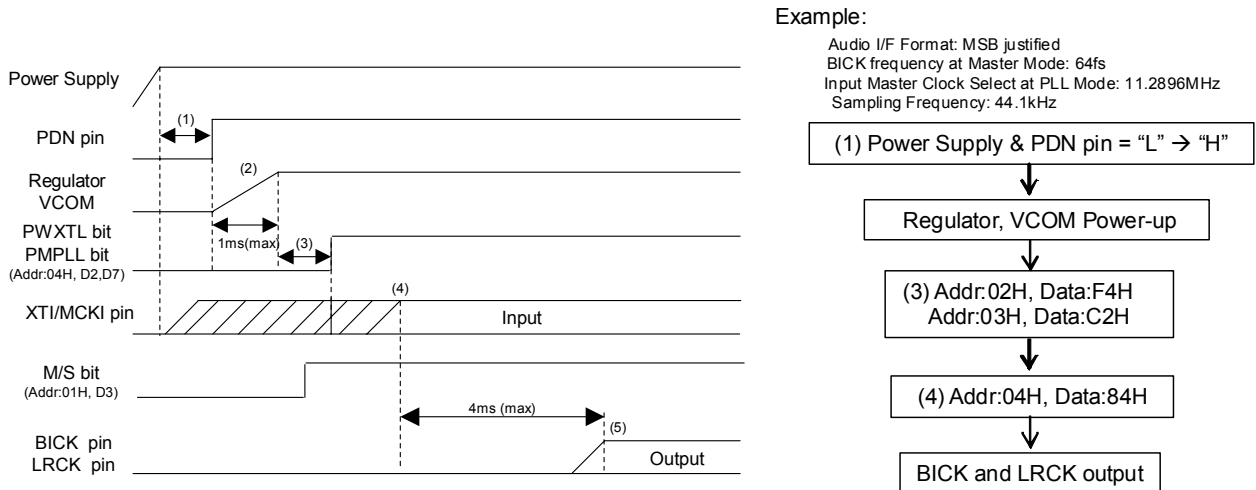
Figure 77. Clock Set Up Sequence (1)
