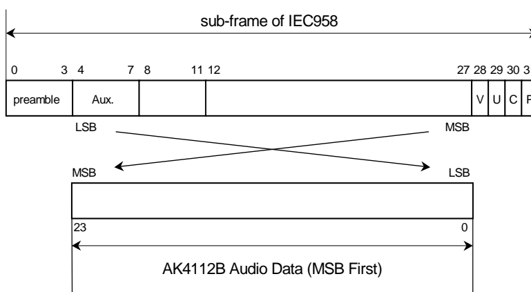
Figure 5. Bit configuration
