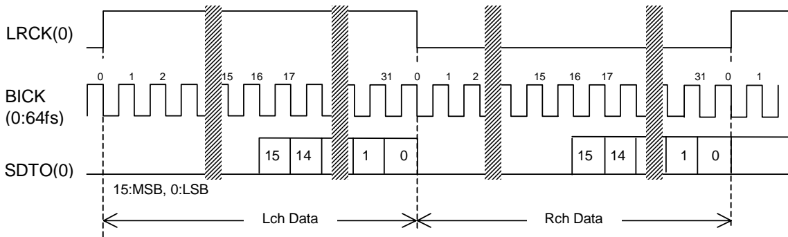
Figure 30. Mode 0 Timing
