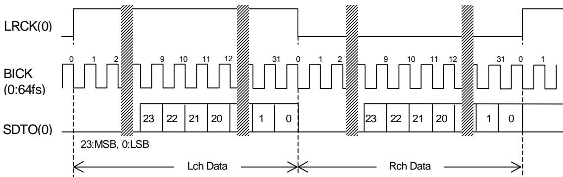
Figure 31. Mode 3 Timing
