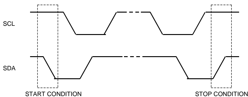
Figure 17. START and STOP conditions
