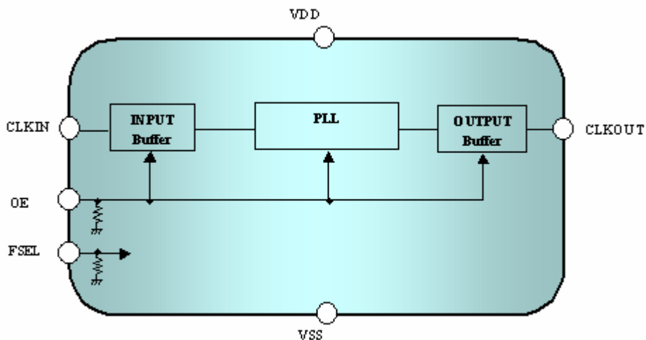
AK8110 Single Clock Generator
