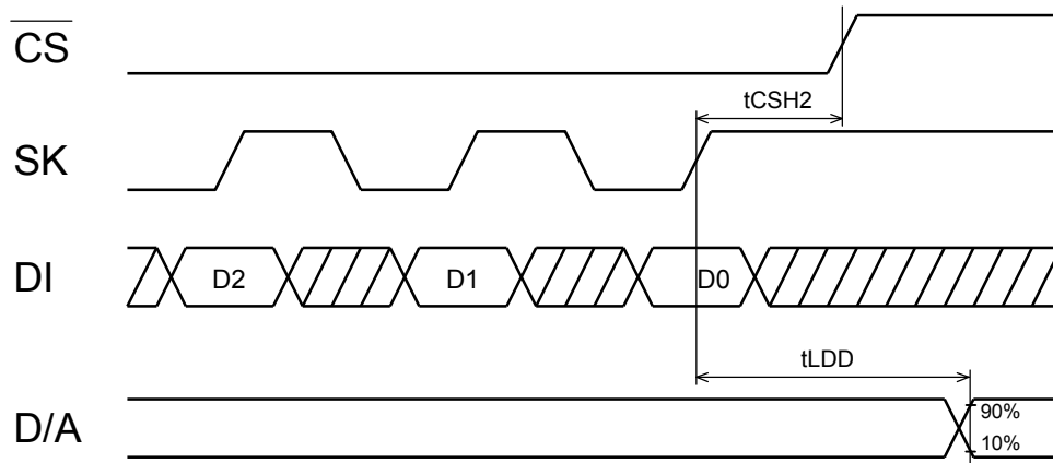
Programming timing in WRITE instruction
