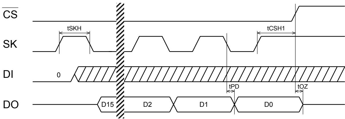
Data latch timing in READ operation
