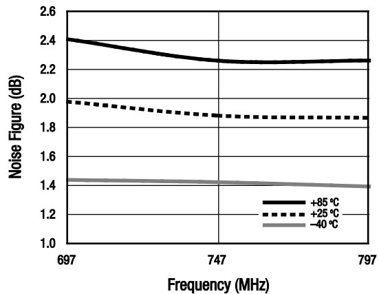
Figure 14. Noise Figure vs Frequency Over Temperature
