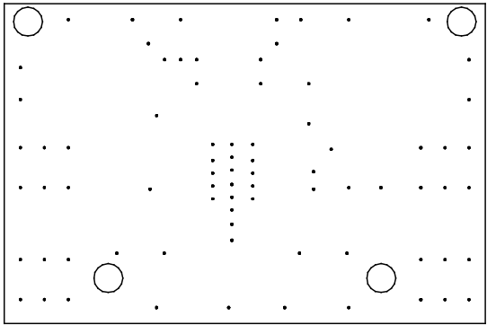
Layer 3: Ground
