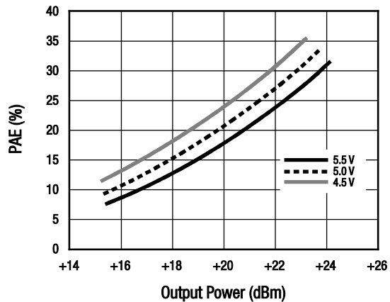
Figure 16. PAE vs Output Power Over VCC
