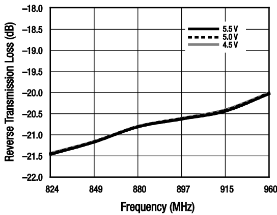
Figure 42. Reverse Transmission Loss vs Frequency Over VCC
