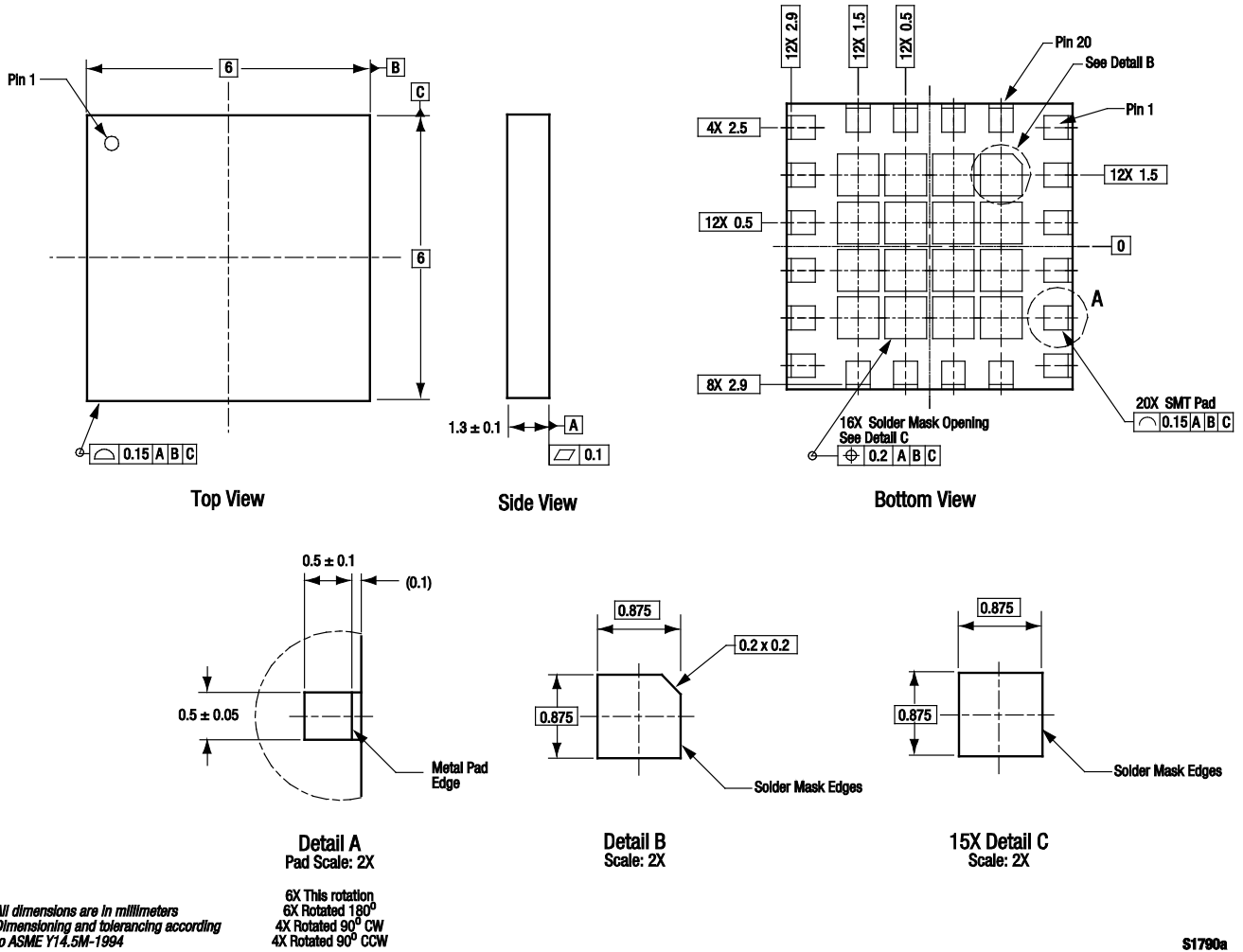
Figure 25. SKY65137-11 20-Pin MCM Package Dimensions
