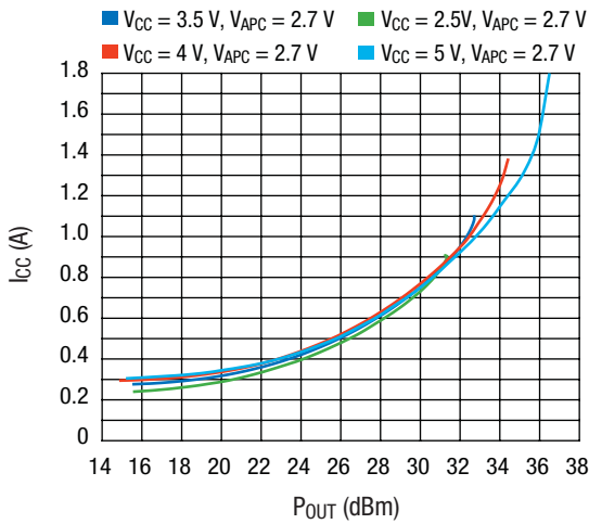
ICC vs. P_{OUT} and V_{CC} , V_{APC1,2} = 2.7\text{ V} , 915 MHz @ 25 °C
