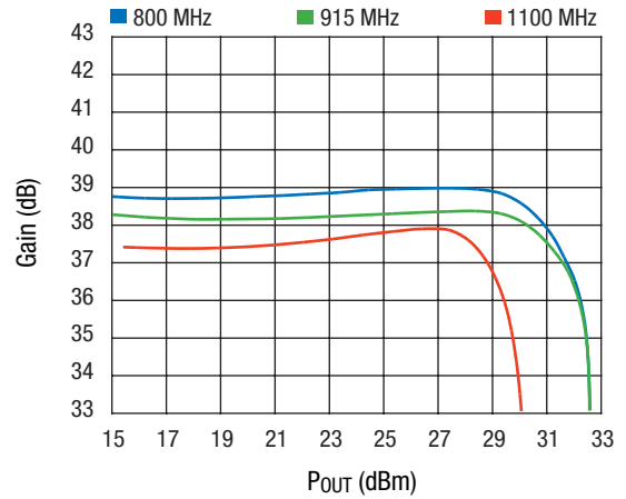
Gain vs. P OUT and Frequency V CC = 3.5, T = 25 °C, V APC1,2 = 2.6 V
