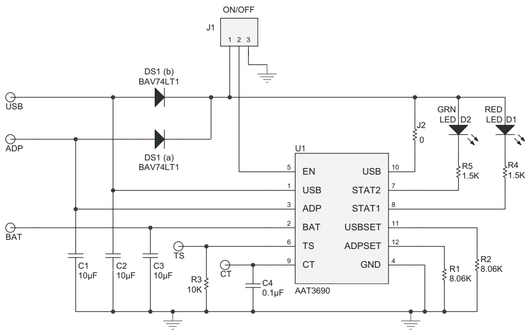
Figure 3: AAT3690 Evaluation Board Schematic.
