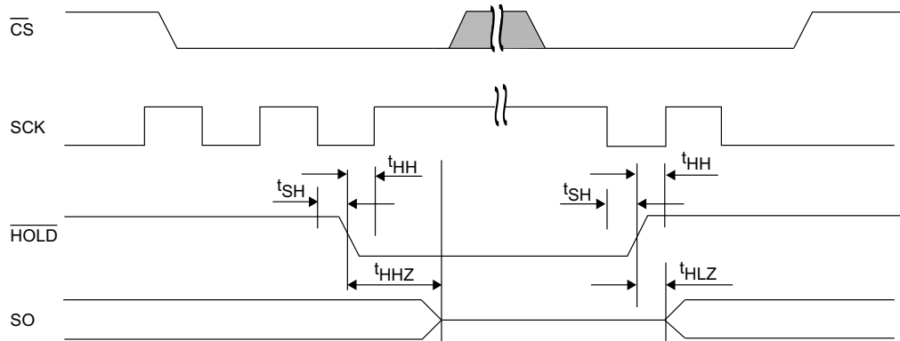
Figure 31. HOLD Timing
