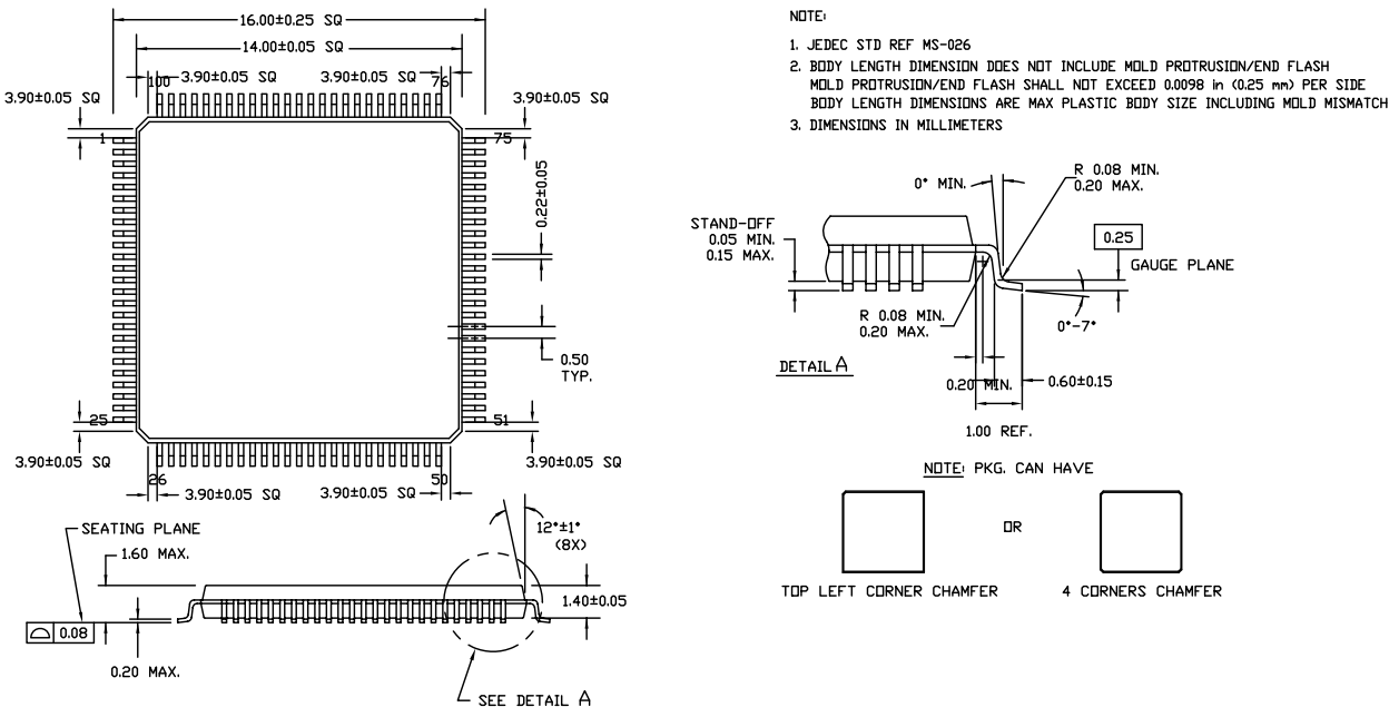
Figure 17. 100-pin TQFP (14 x 14 x 1.4 mm) A100SA Package Outline, 51-85048
