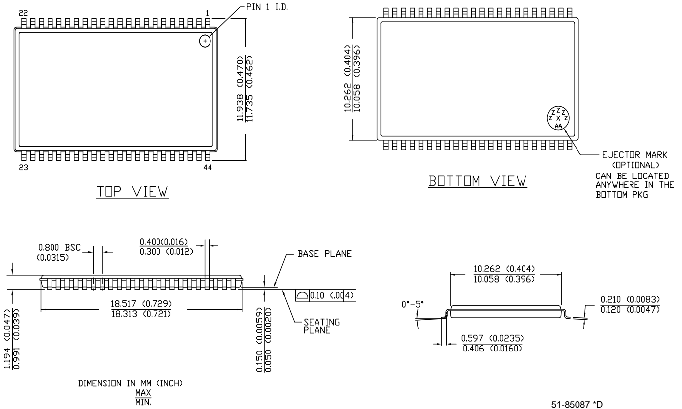
Figure 2. 44-pin TSOP Z44-II, 51-85087
