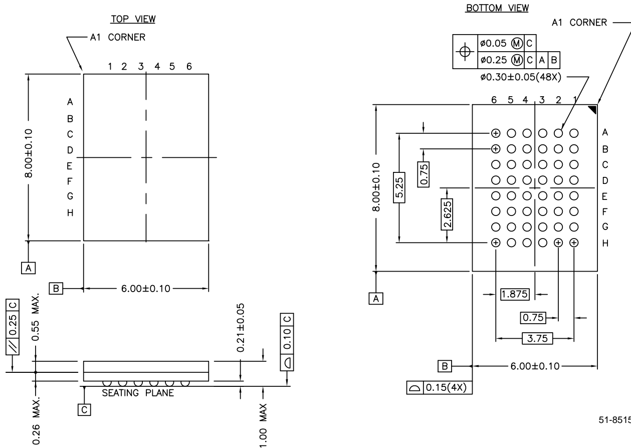
Figure 6. 48-pin VFBGA ( 6 \times 8 \times 1 mm) BV48/BZ48, 51-85150
