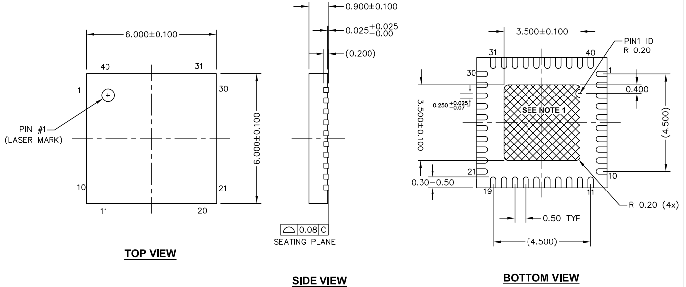
Figure 12. 40-Pin Sawn QFN (6 x 6 x 0.90 mm)
