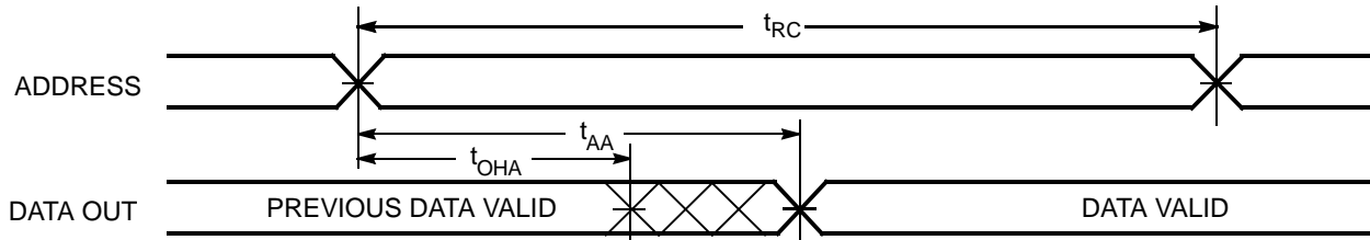
Figure 3. Read Cycle 2 ( \overline{\text{OE}} Controlled) [19, 20]
