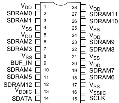
Figure 1. 28-pin SOIC (Top View)
