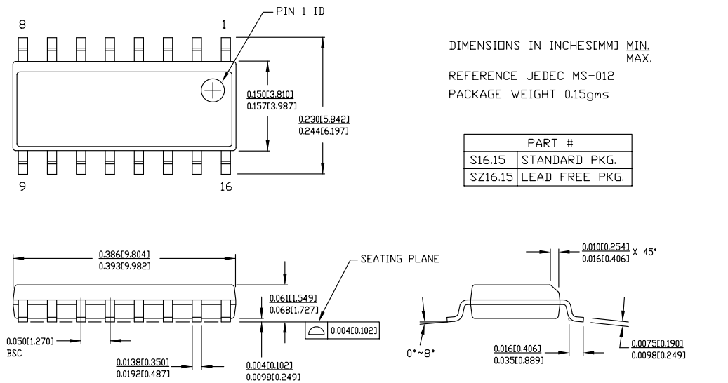
Figure 10. 16-Pin (150-Mil) SOIC S16 and SZ16
