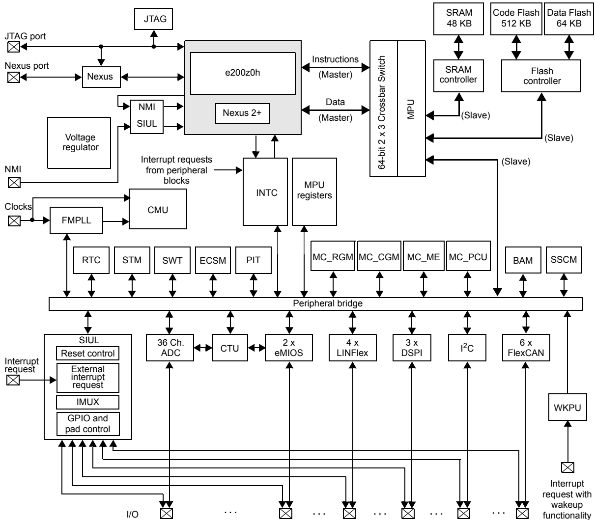
Figure 1. MPC5604B/C block diagram
