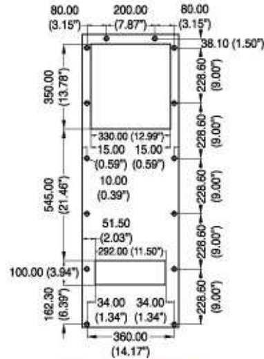
Drilling Template
