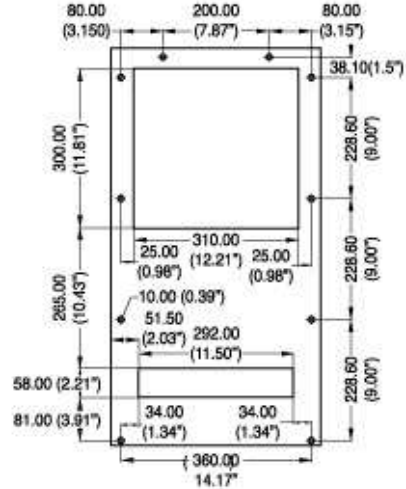
Drilling Template
