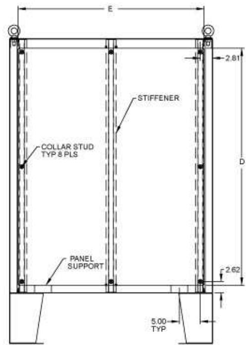
SECTION Y-Y
