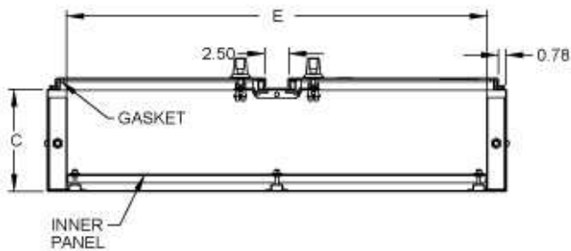
SECTION X-X
