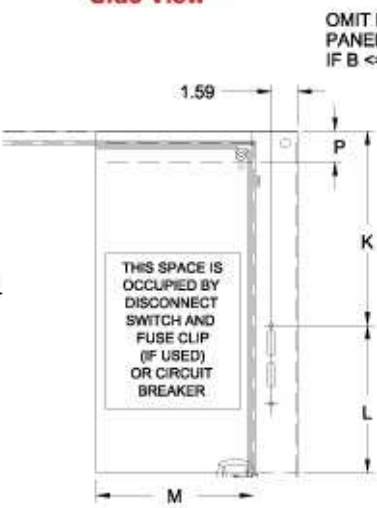
Disconnect Mounting Details
