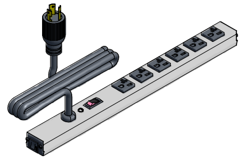
ISOMETRIC VIEW
