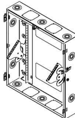
PERSPECTIVE VIEW (DOOR REMOVED)
