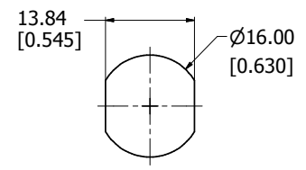
PANEL CUTOUT (NOT TO SCALE)
