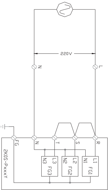
FIG. B: 1Ø 220VAC SYSTEM
