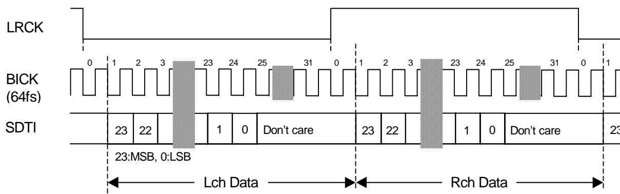
Figure 4. Mode 3 Timing
