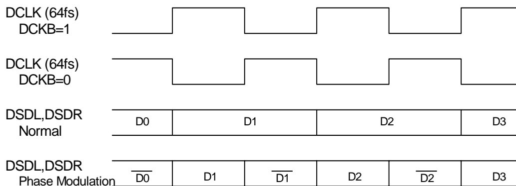
Figure 11. DSD Mode Timing
