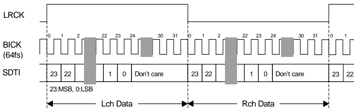
Figure 3. Mode 2 Timing
