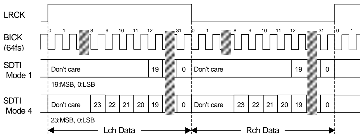
Figure 2. Mode 1,4 Timing
