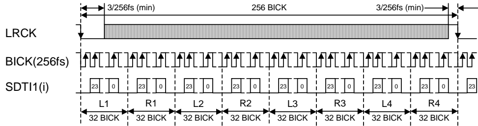
Figure 6. Mode 6 Timing
