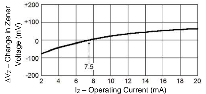
FIGURE 4 TYPICAL CHANGE OF ZENER VOLTAGE WITH CHANGE IN OPERATING CURRENT
