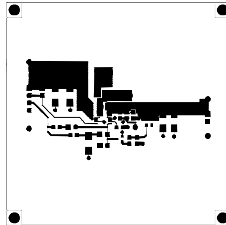
Figure 6 – LX1742 - Evaluation Board Trace Layout
