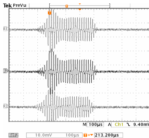
Figure 8- Output current during digital dimming with 5% duty cycle R1= i out (Master) R2=i out (Slave1) R3=i out (Slave2) Lamp Current at 10mA/Div
