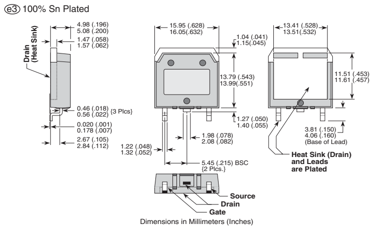
Dimensions in Millimeters (Inches)
