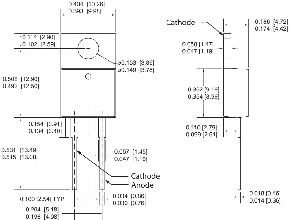
Dimensions in Millimeters and (Inches)
