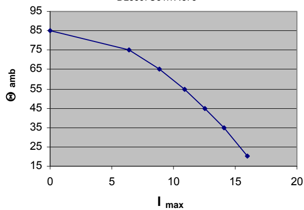
Max. allowable ambient Temp. at specific current (rms) B25667C3147A375
