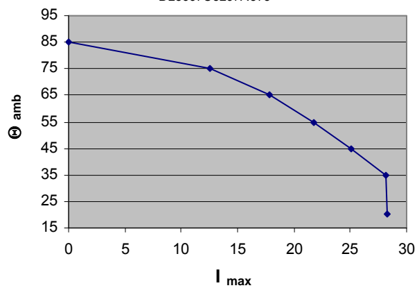
Max. allowable ambient Temp. at specific current (rms) B25667C3297A375
