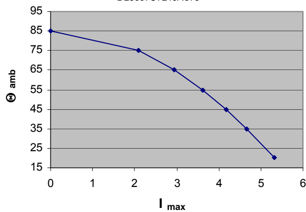
Max. allowable ambient Temp. at specific current (rms) B25667C7246A375
