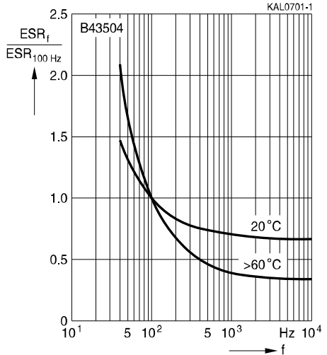
Frequency characteristics of ESR Typical behavior
